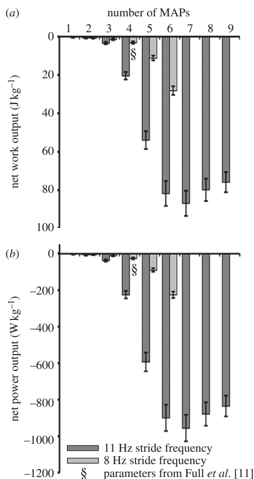
Figure 4. Activation sweep. (a) Work and (b) power outputs from dynamic oscillations of stimulated muscle 137 in the intact-joint work loop preparation showed primarily energy absorbing outcomes as activation was increased. Increasing cycle frequency (8 Hz stride frequency; light grey bars) from those of past studies [11] to the stride frequency observed in our in vivo experiments (11 Hz stride frequency; dark grey bars) increased energy absorption. Intact-joint work loops using the same parameters as previously published [11] isolated muscle work loops produced statistically indistinguishable work and power (bars marked with §).
