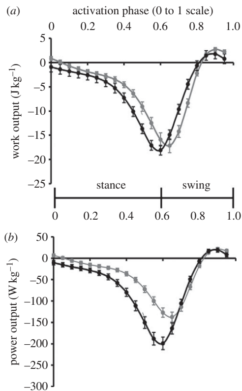
Figure 5. Work loop phase dependency. The ventral femoral extensor (a) work and (b) power outputs depended on phase of activation when the strain parameters remained unchanged (figure 1b(iv)). Typical phase of activation during steady running is approximately 0.05–0.1 [17]. The shape of the phase response curves was comparable to isolated muscle phase responses [11], reaching a minimum when stimulus onset was close to the swing–stance transition at 0.6 (60% duty factor). Increasing stride frequency (11 Hz stride frequency, black lines versus 8 Hz stride frequency, grey lines) had different effects when the stimulus phase was in stance or swing and shifted the peak of energy absorption (curve minima).
