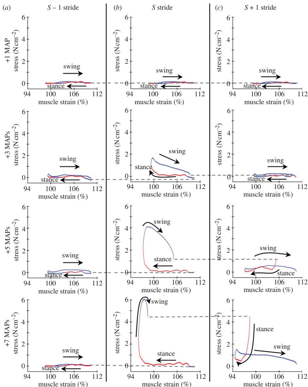
Figure 7. Work loops from the burst extension trials. Work loop output for (a) S - 1 , (b) S and (c) S + 1 strides under each neural feedback condition (one, three, five or seven added MAPs, top to bottom) show how this muscle is recruited to do positive work in addition to enhanced negative work (figure 6). The S - 1 stride was not significantly different from a typical stride because activation only extended forward in time. Adding MAPs resulted in significant stress during the end of S stride stance and persisting through swing (b, bottom plots). This resulted in enhanced positive work production at the very end of S stride stance (rising red line), increased negative work throughout swing (blue line) and the increased positive work at the onset of the S + 1 stride (red line).
