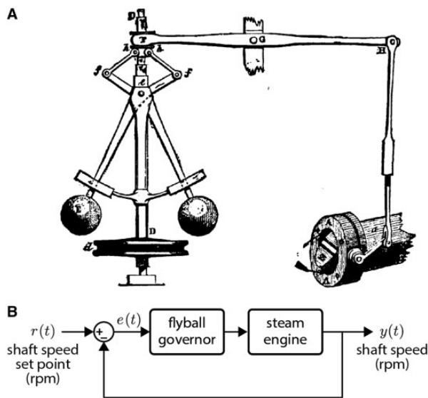
Fig. 1 (A) Schematic of the Watt–Boulton centrifugal “flyable” governor (copyright expired; see http://copyright.cornell.edu/resources/publicdomain.cfm ) and (B) a simplified feedback diagram.
