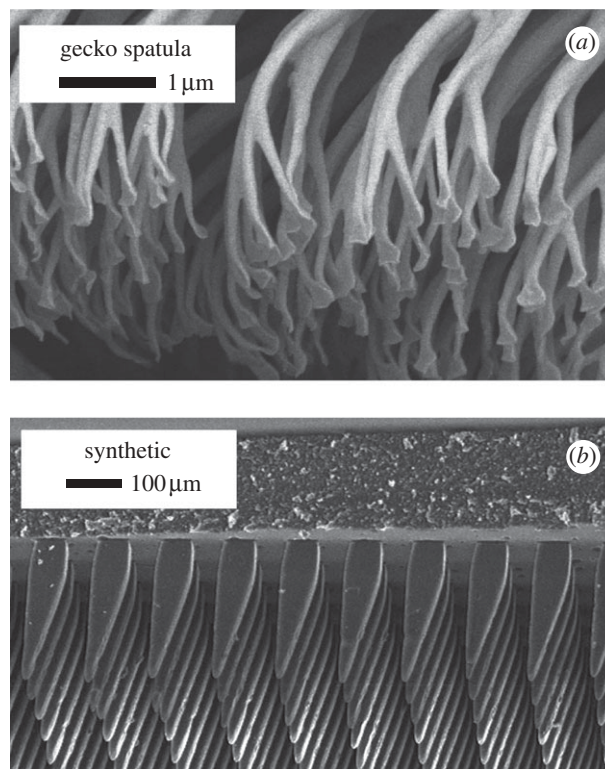
Figure 5. Fibrillar geometry of (a) natural gecko setae and (b) GSA.
